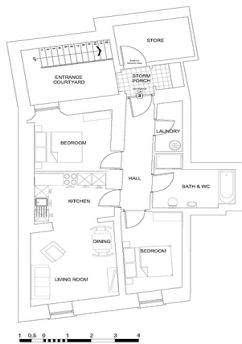
Lower Ground Floor Plan
